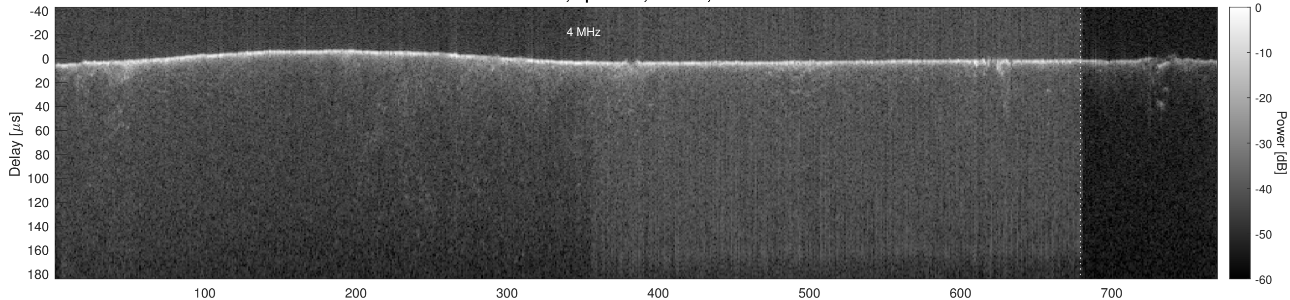
Orbit 22546, Optimized, Window, Channel 2
