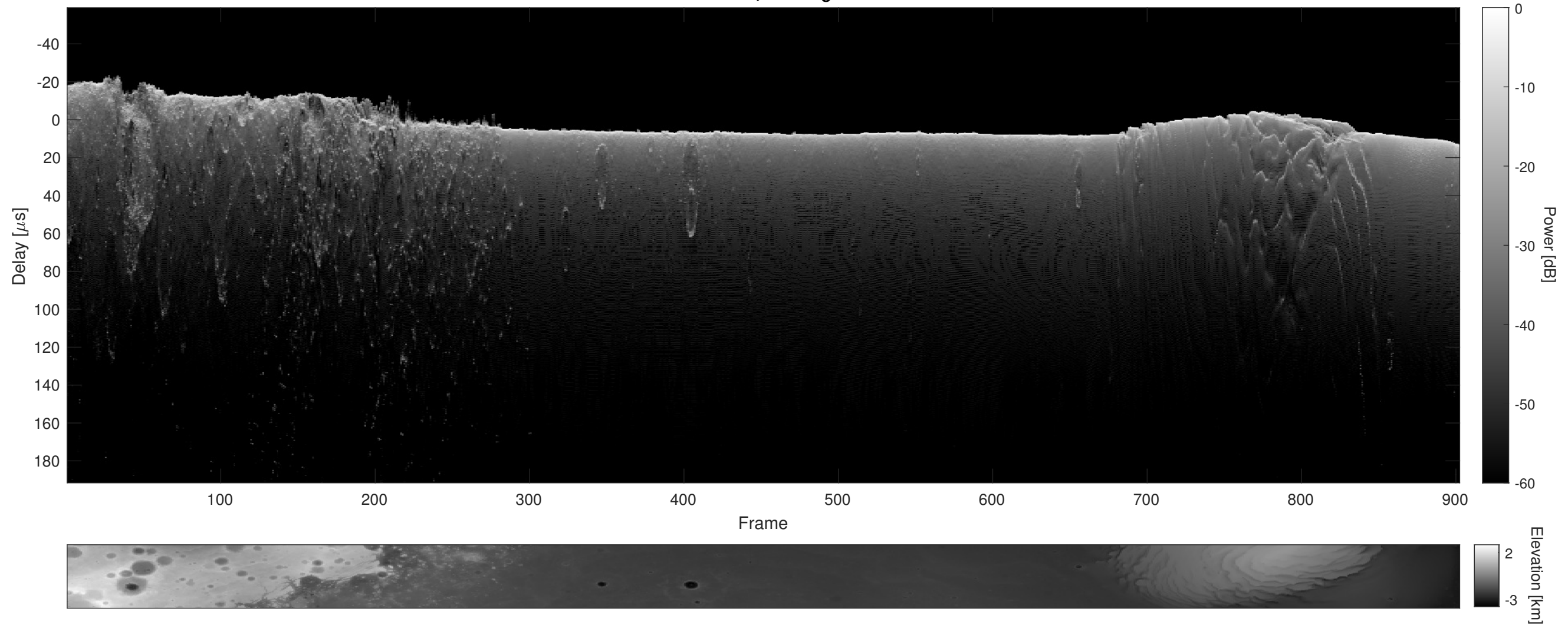
Orbit 22547, Cluttergram
