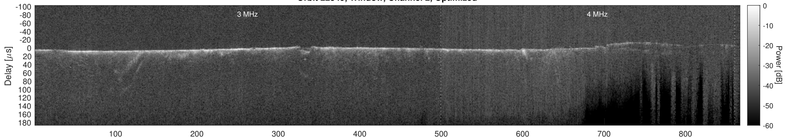
Orbit 22549, Cluttergram
