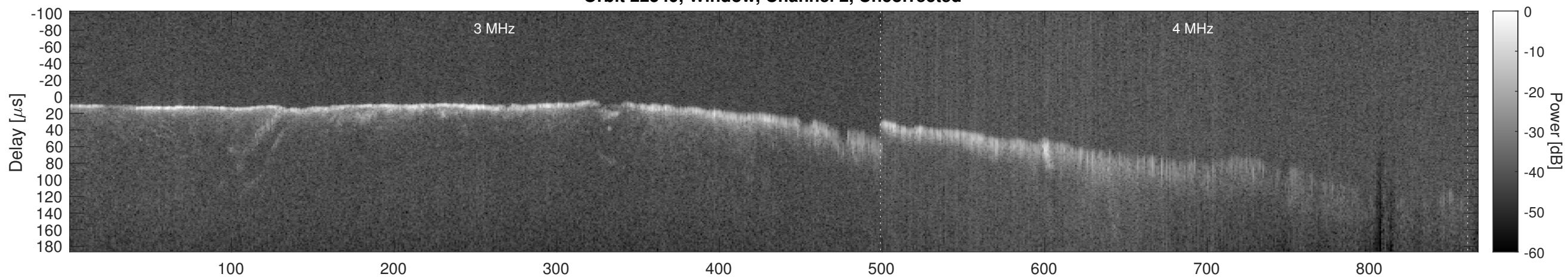
Orbit 22549, Window, Channel 2, Chapman
