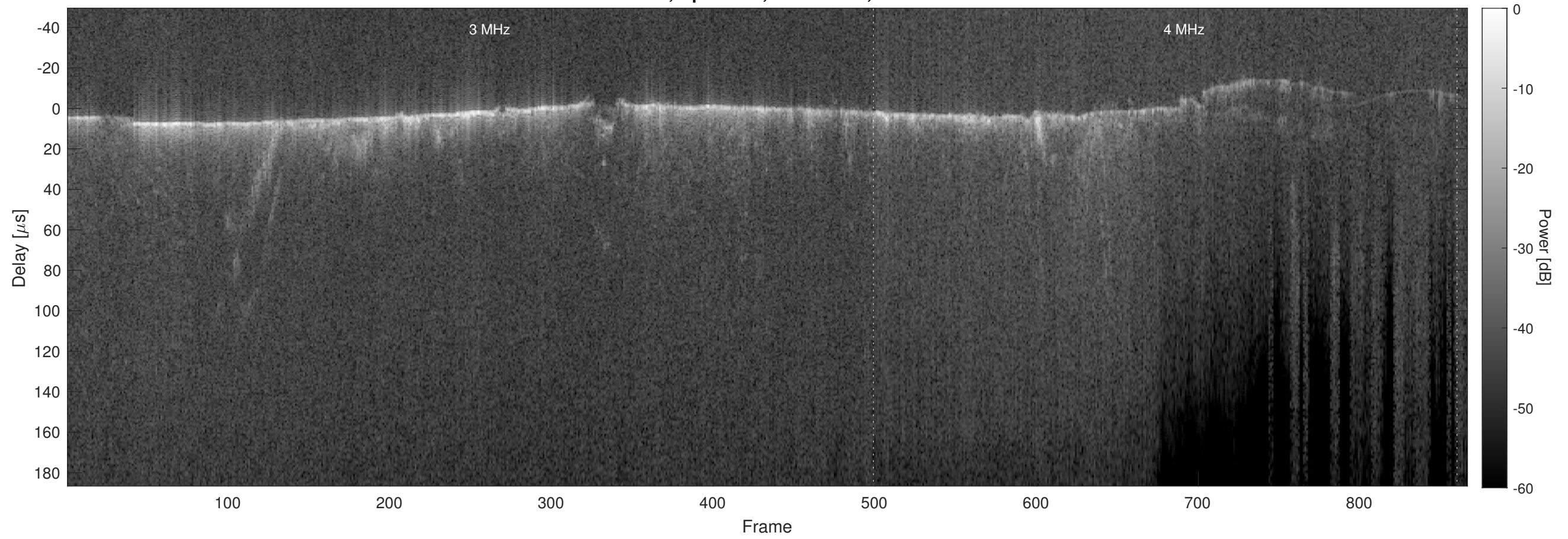
Orbit 22549, Optimized, No Window, Channel 2
