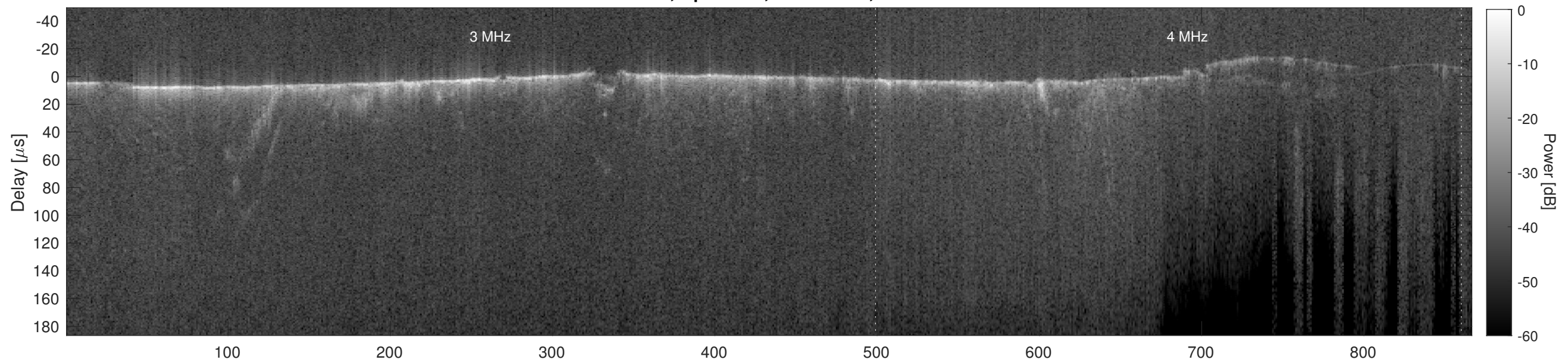
Orbit 22549, Cluttergram
