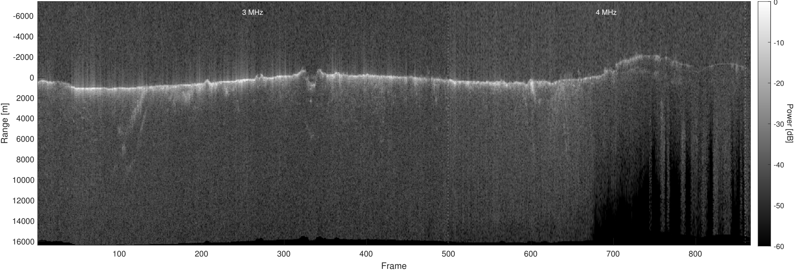
Orbit 22549, Optimized, No Window, Depth-Corrected, Channel 2
