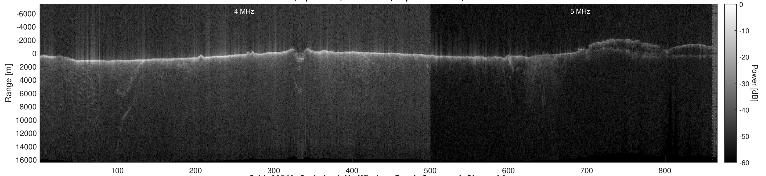
Orbit 22549, Optimized, No Window, Depth-Corrected, Channel 2
