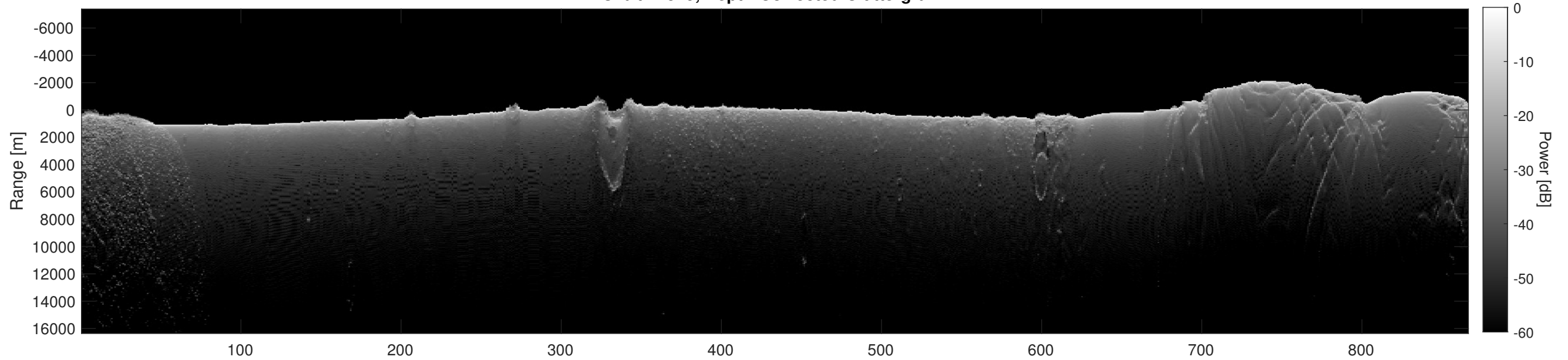
Orbit 22549, Depth-Corrected Cluttergram
