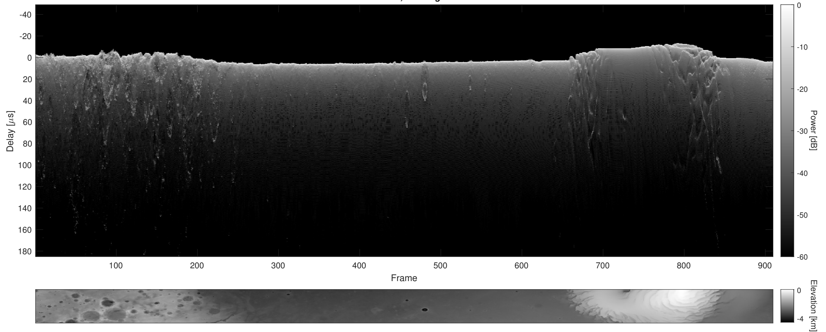
Orbit 22551, Cluttergram
