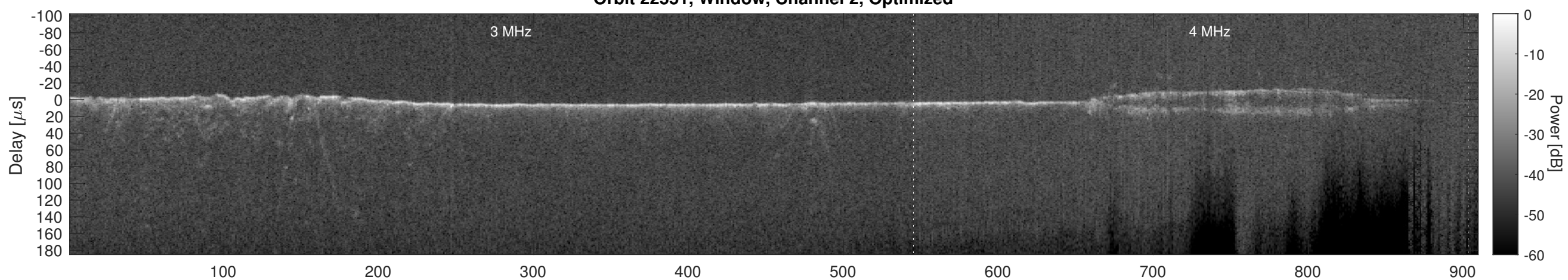
Orbit 22551, Cluttergram
