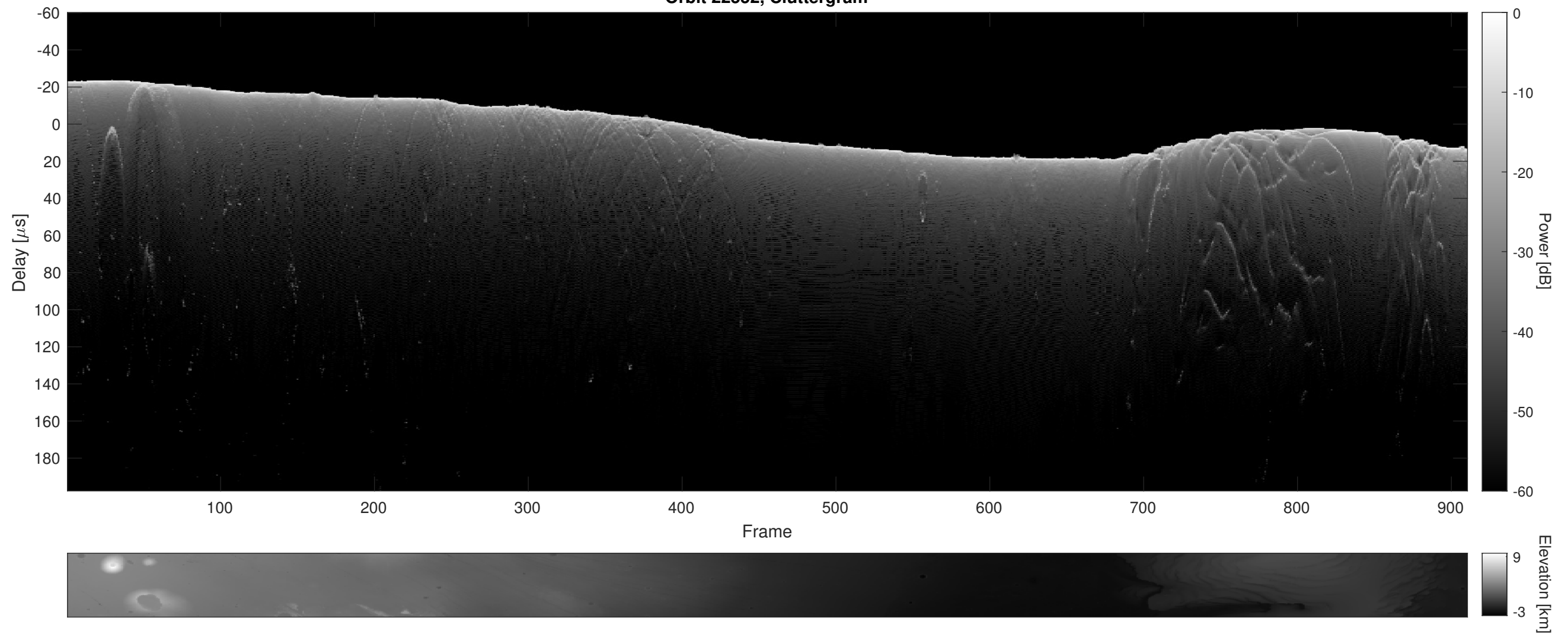
Orbit 22552, Cluttergram
