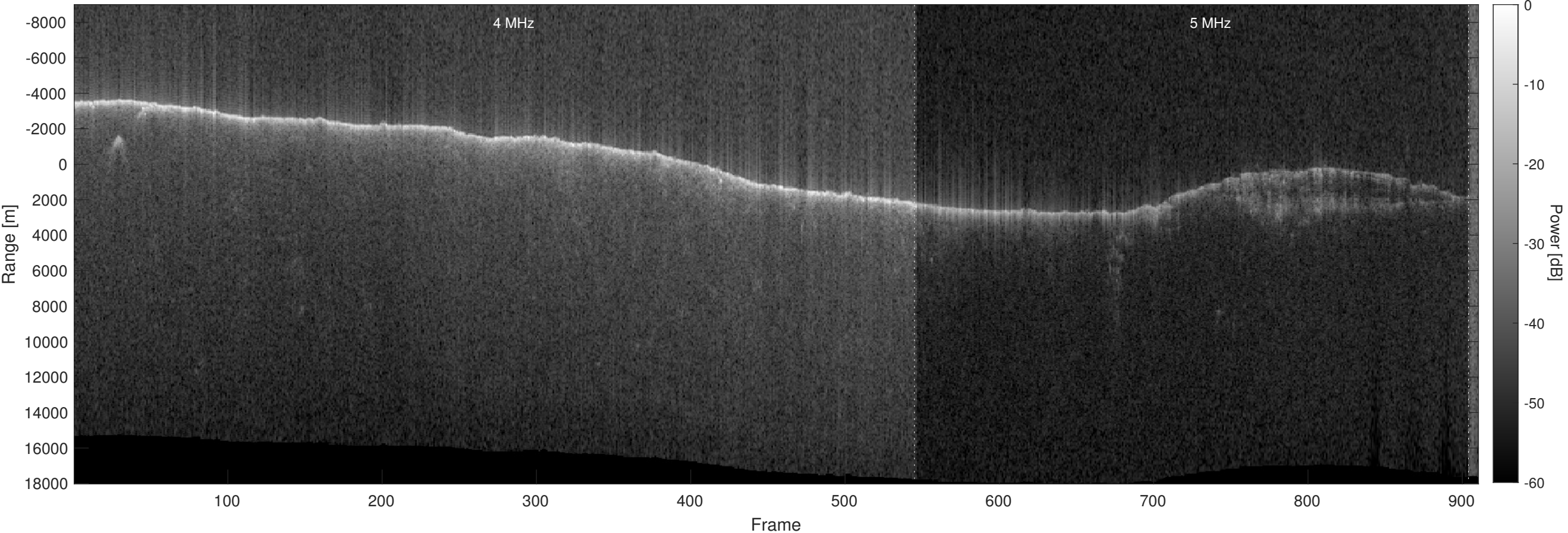
Orbit 22552, Optimized, No Window, Depth-Corrected, Channel 2
