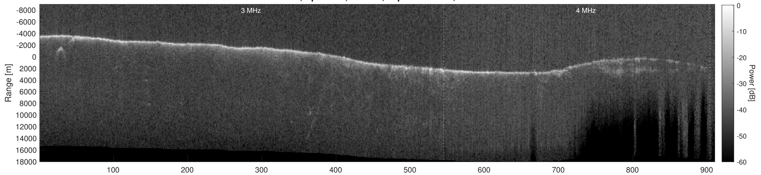
Orbit 22552, Depth-Corrected Cluttergram
