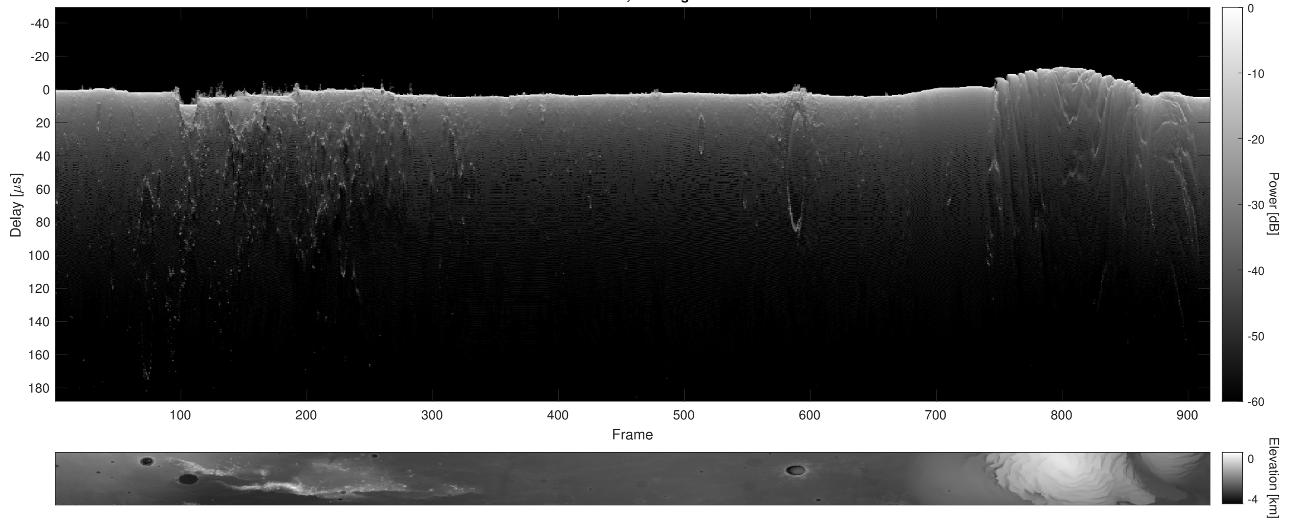
Orbit 22553, Cluttergram
