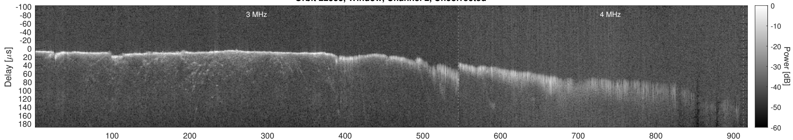
Orbit 22553, Window, Channel 2, Chapman
