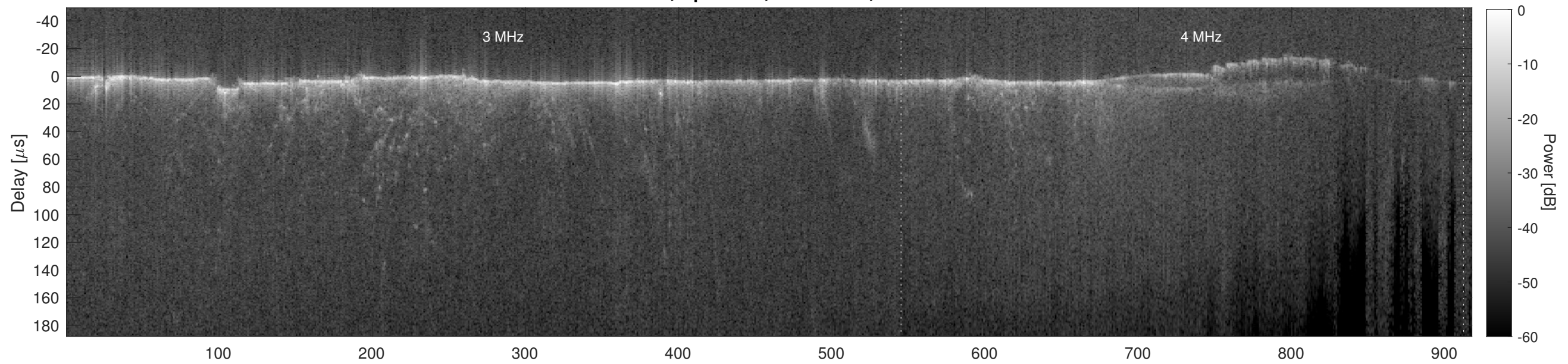
Orbit 22553, Cluttergram
