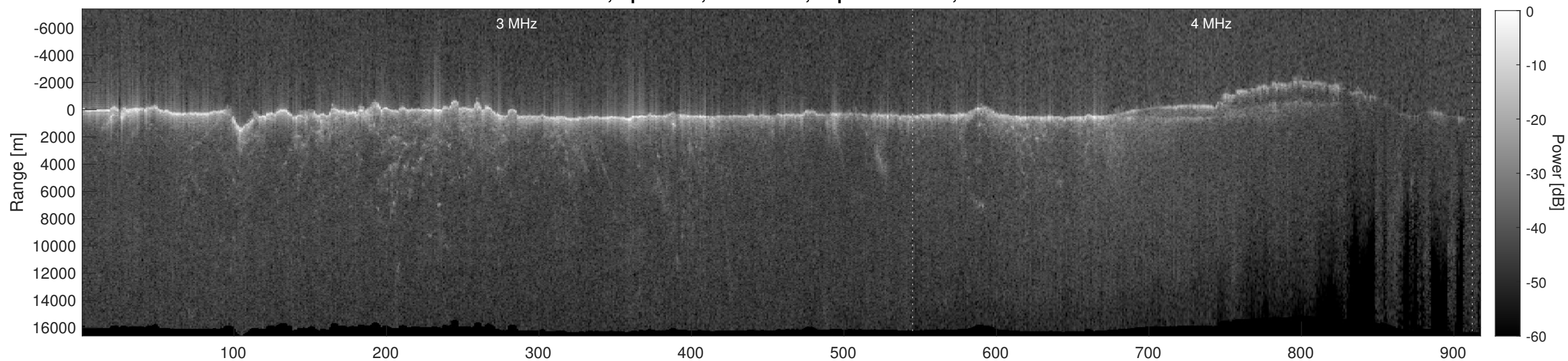
Orbit 22553, Depth-Corrected Cluttergram
