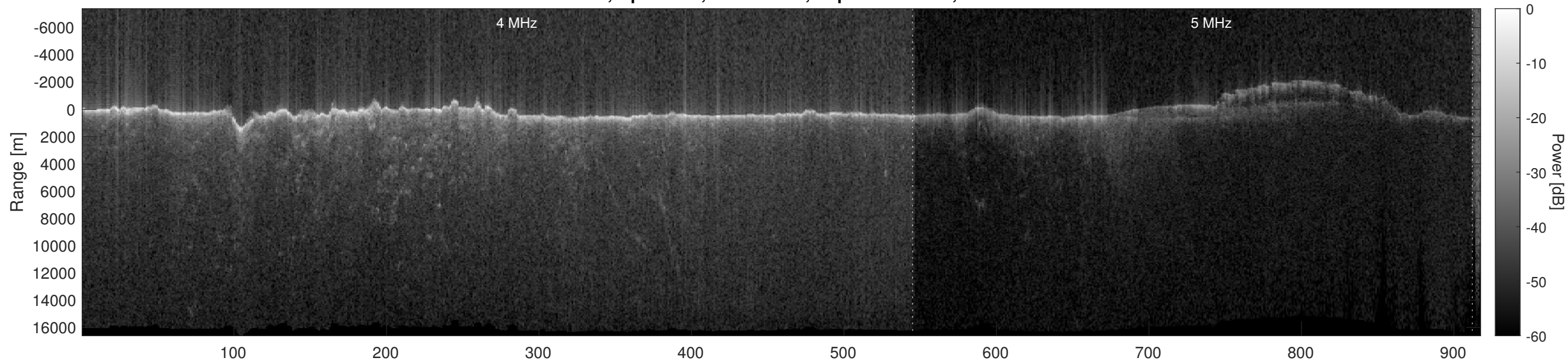
Orbit 22553, Optimized, No Window, Depth-Corrected, Channel 2
