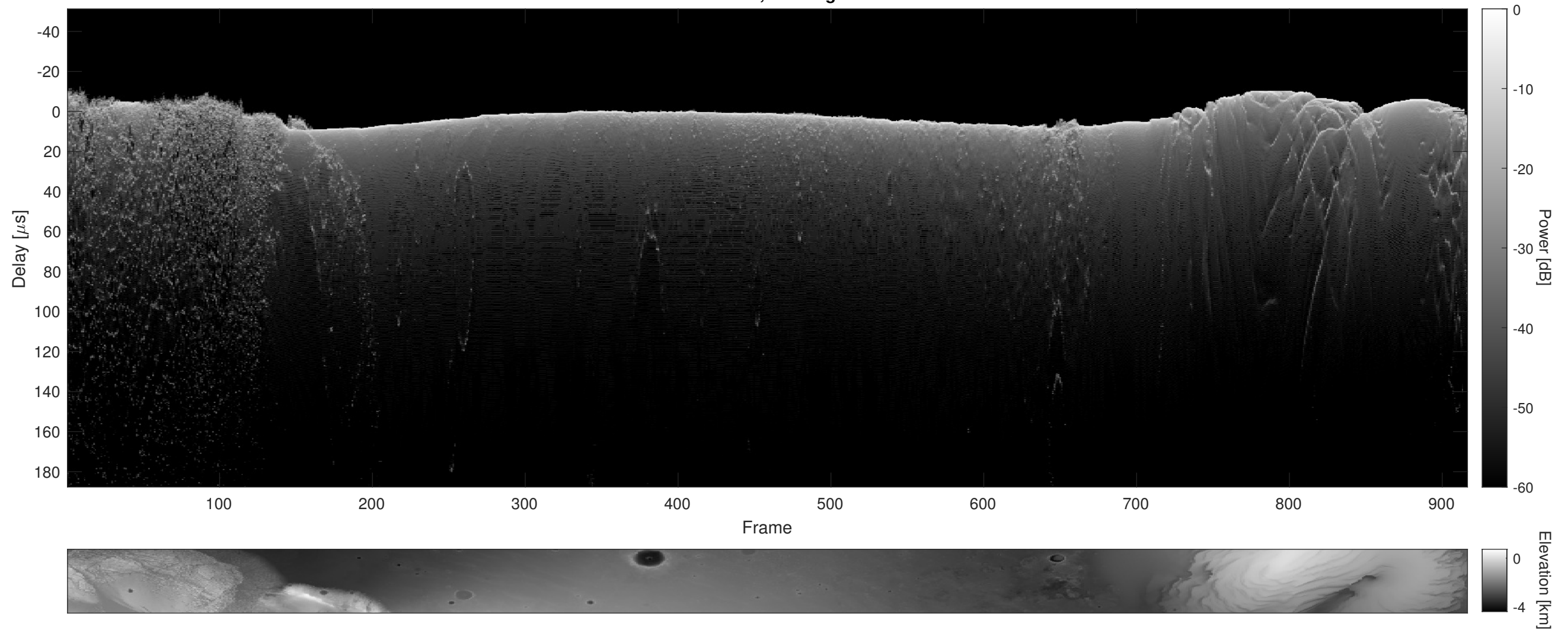
Orbit 22556, Cluttergram
