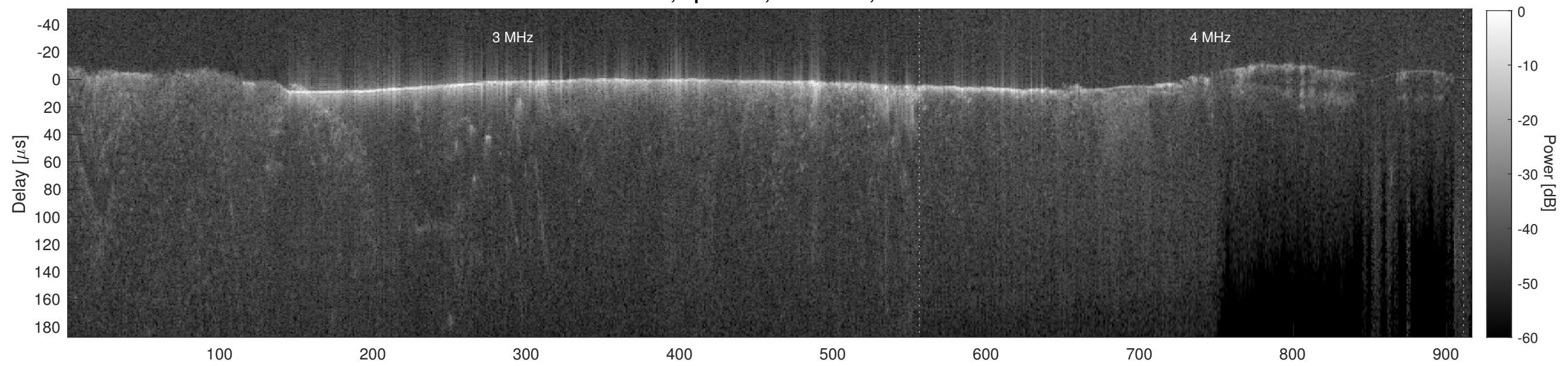
Orbit 22556, Cluttergram
