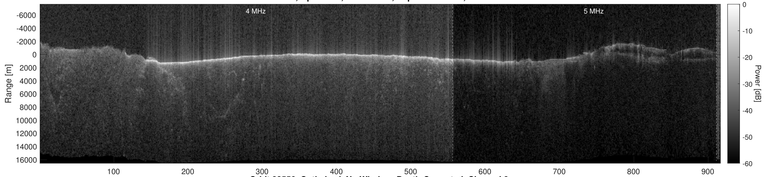
Orbit 22556, Optimized, No Window, Depth-Corrected, Channel 2
