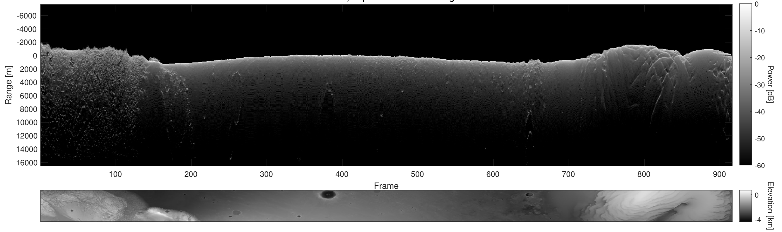
Orbit 22556, Depth-Corrected Cluttergram
