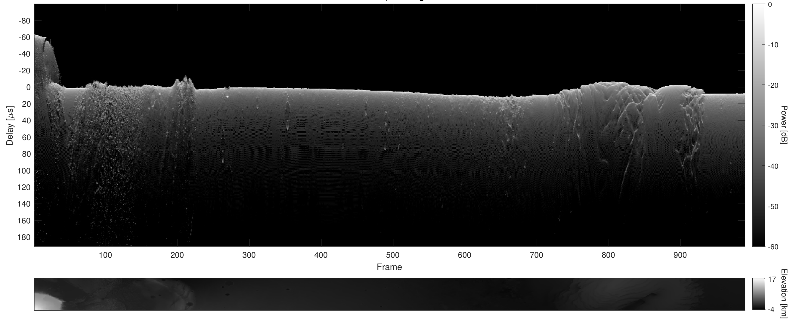
Orbit 22563, Cluttergram
