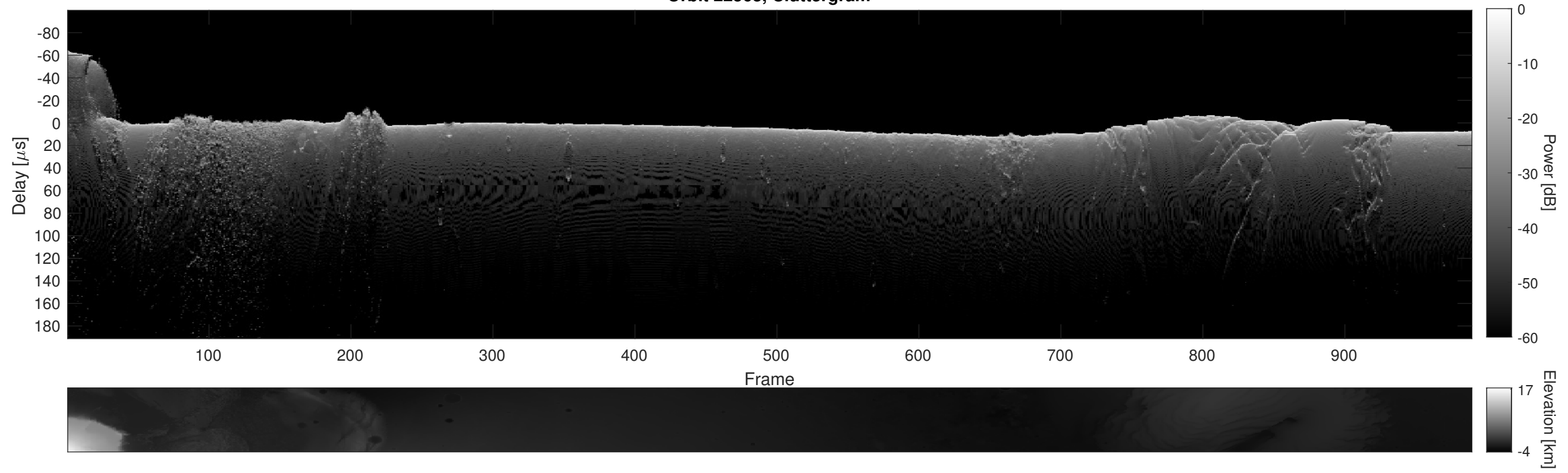
Orbit 22563, Cluttergram
