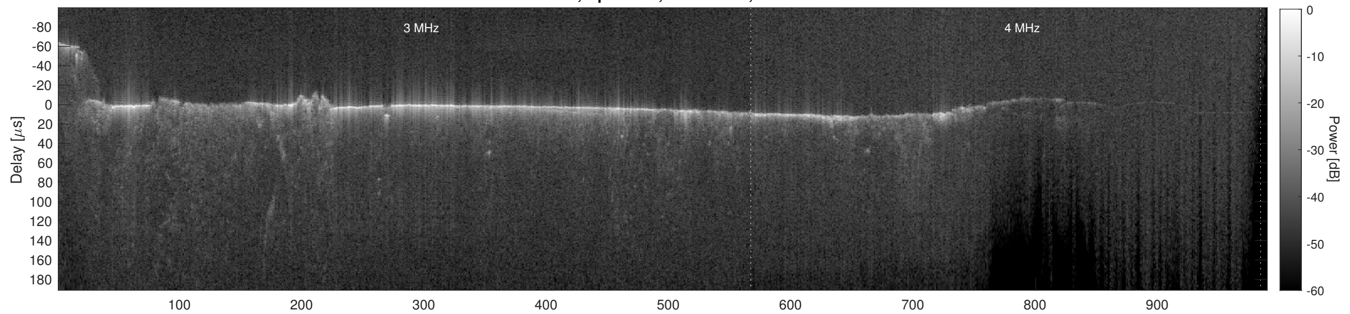
Orbit 22563, Cluttergram
