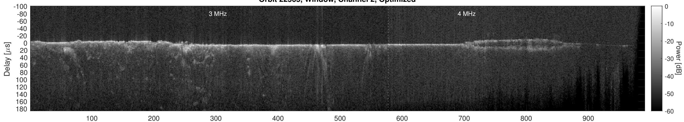
Orbit 22565, Cluttergram
