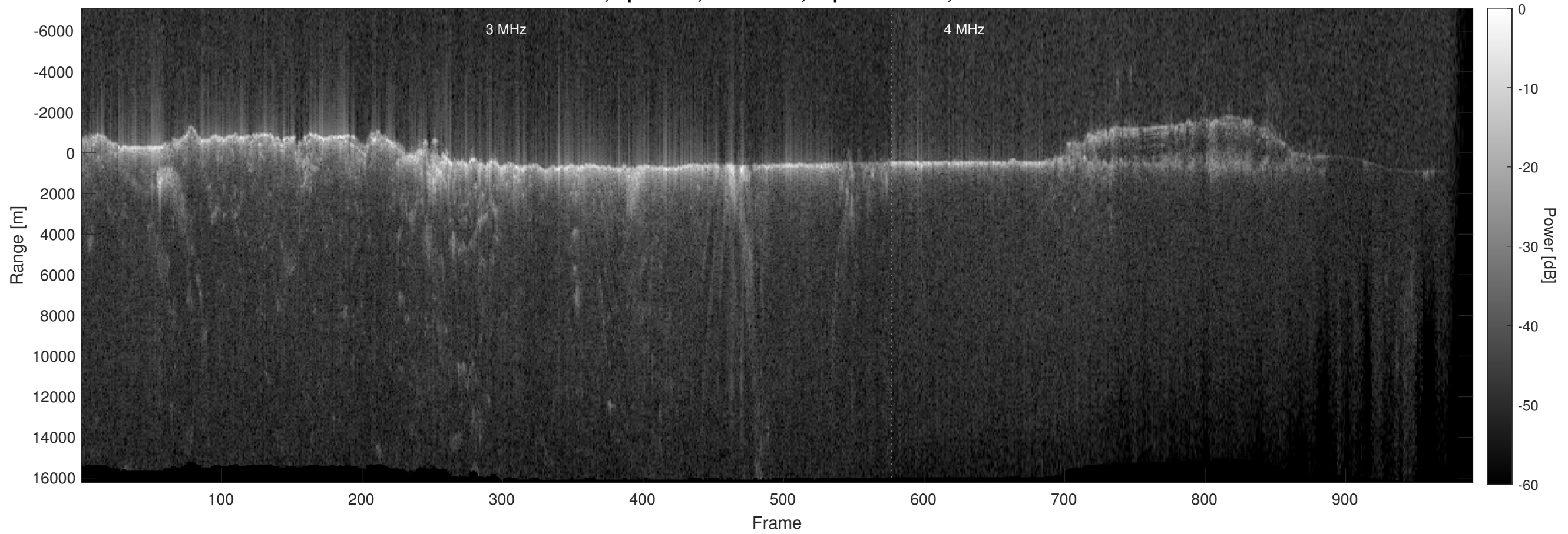
Orbit 22565, Optimized, No Window, Depth-Corrected, Channel 2
