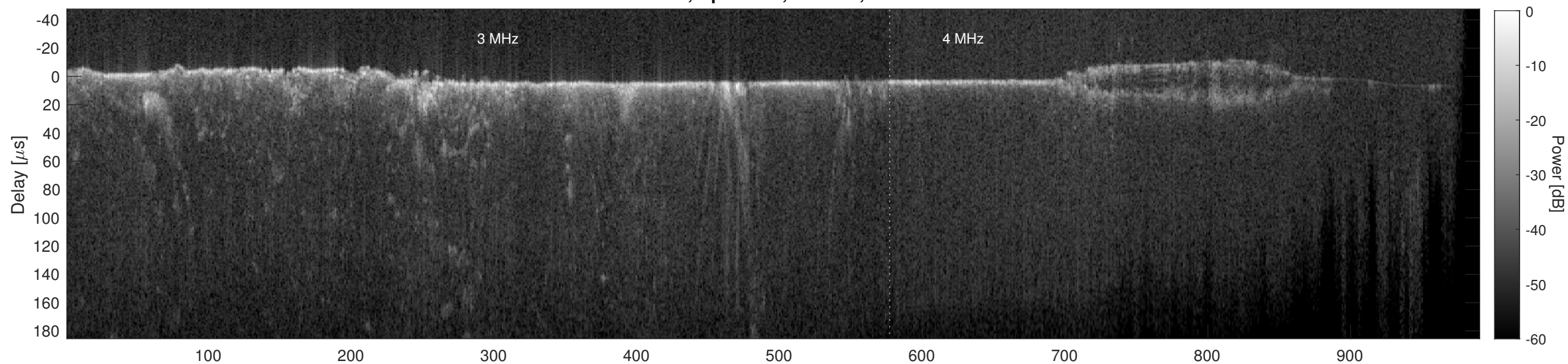
Orbit 22565, Cluttergram
