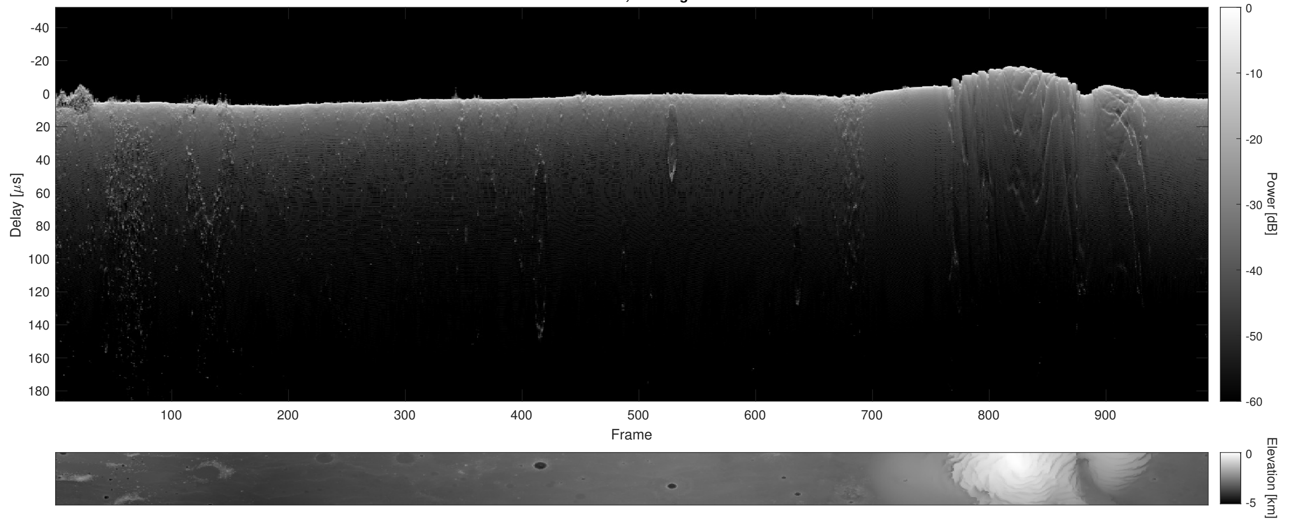
Orbit 22567, Cluttergram
