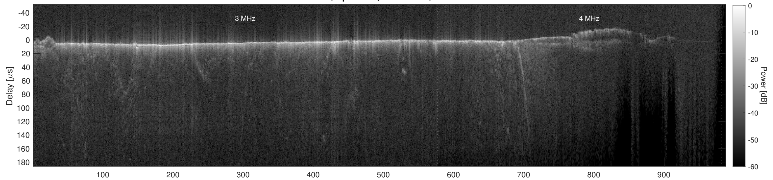
Orbit 22567, Cluttergram
