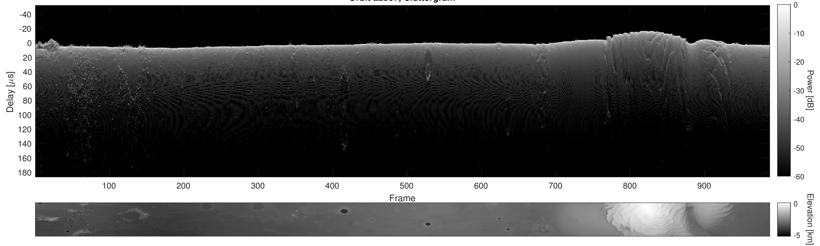
Orbit 22567, Cluttergram
