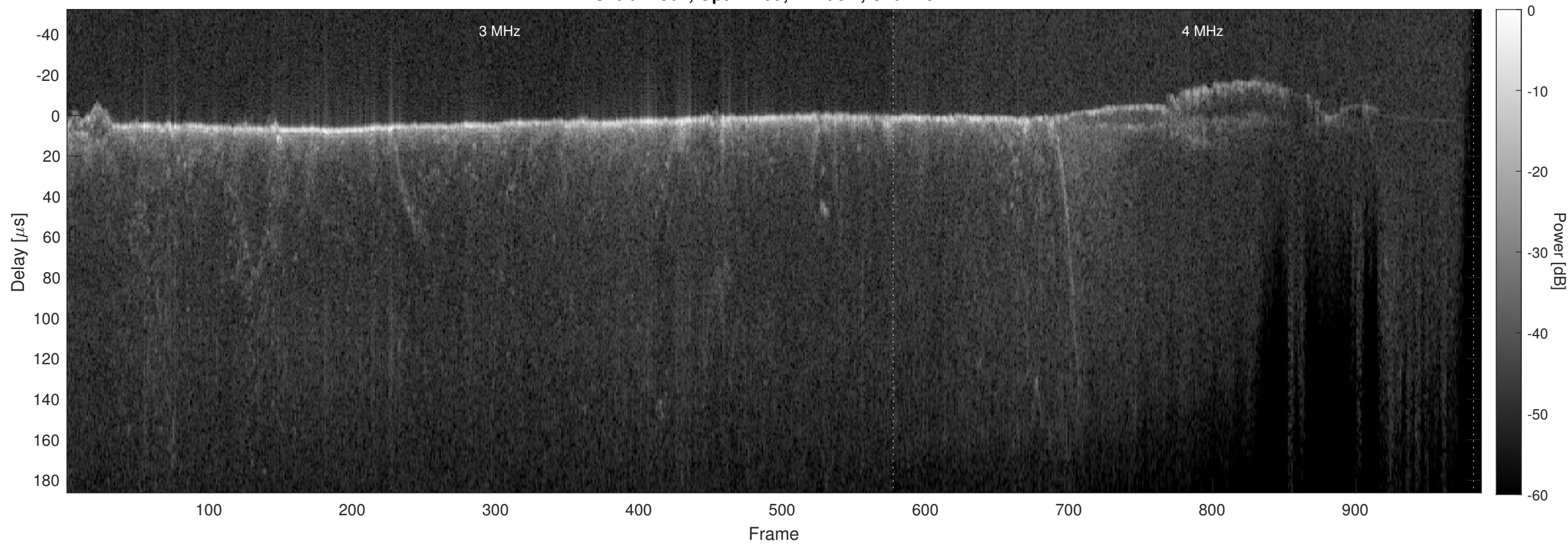
Orbit 22567, Optimized, Window, Channel 2
