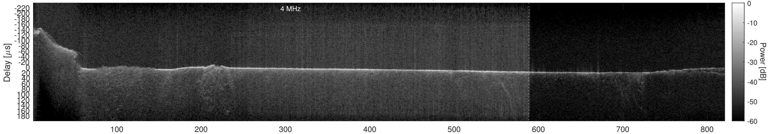
Orbit 22570, Cluttergram
