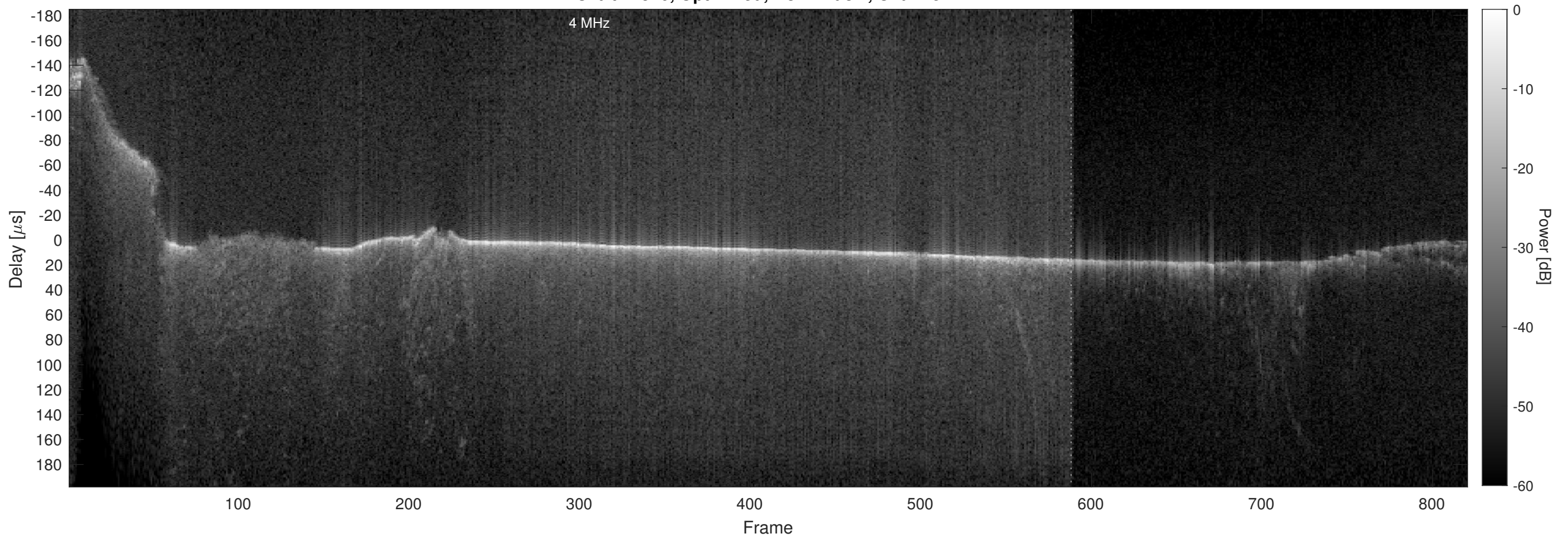
Orbit 22570, Optimized, No Window, Channel 2
