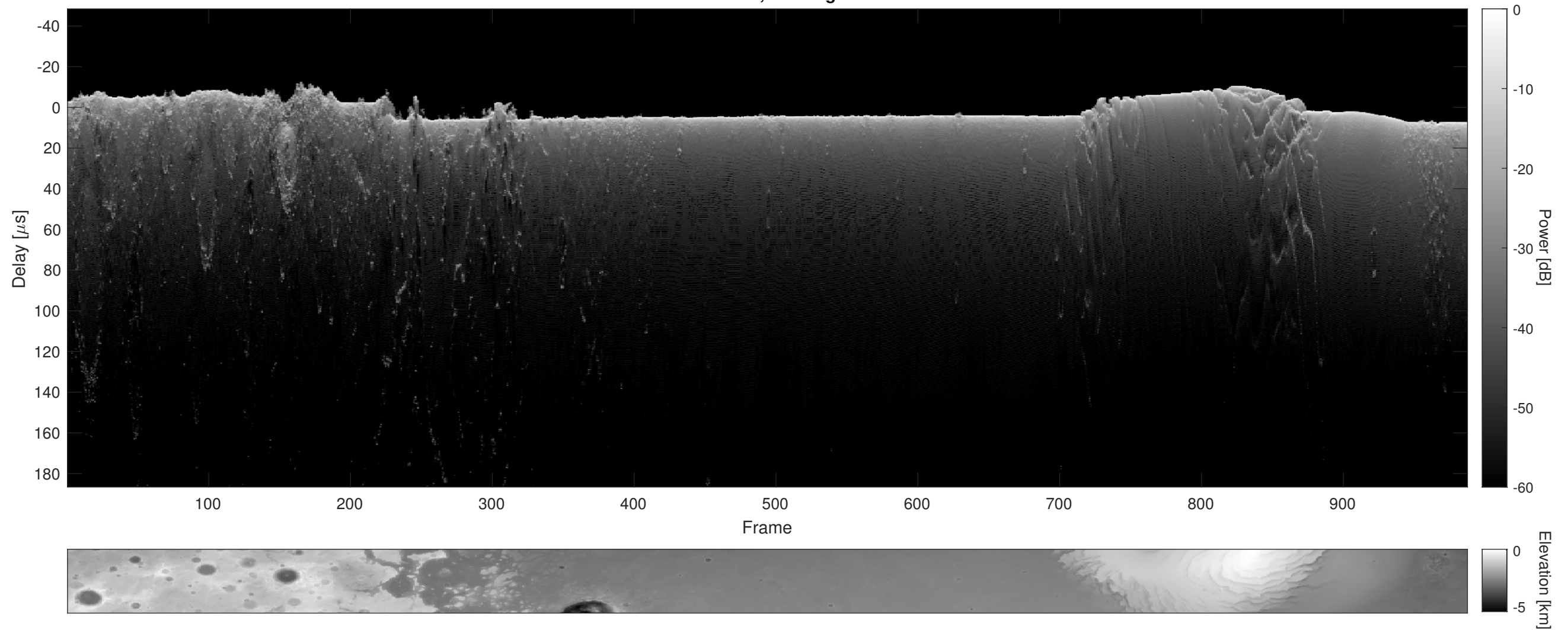
Orbit 22572, Cluttergram
