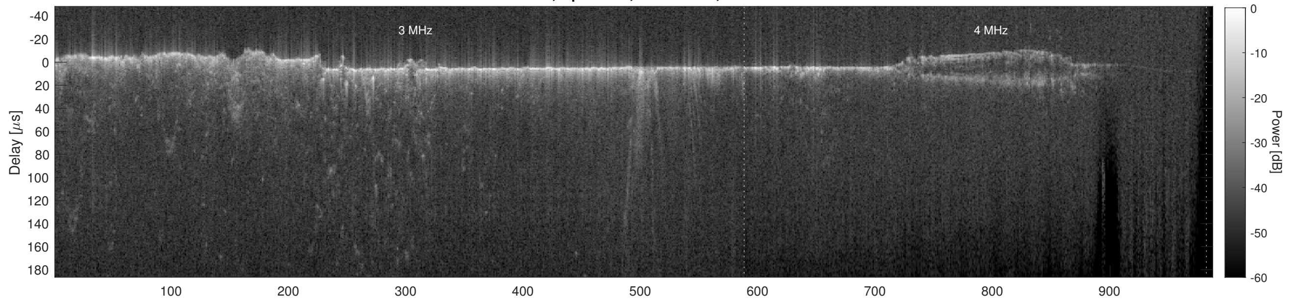
Orbit 22572, Cluttergram
