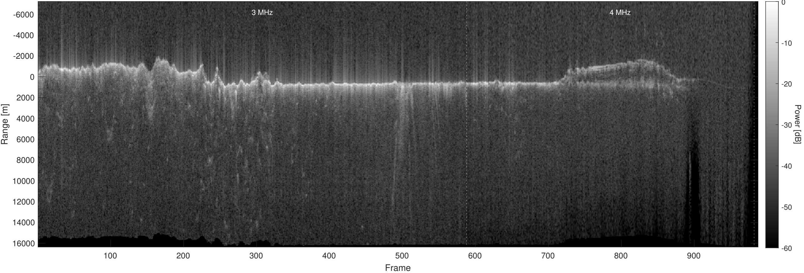
Orbit 22572, Optimized, No Window, Depth-Corrected, Channel 2
