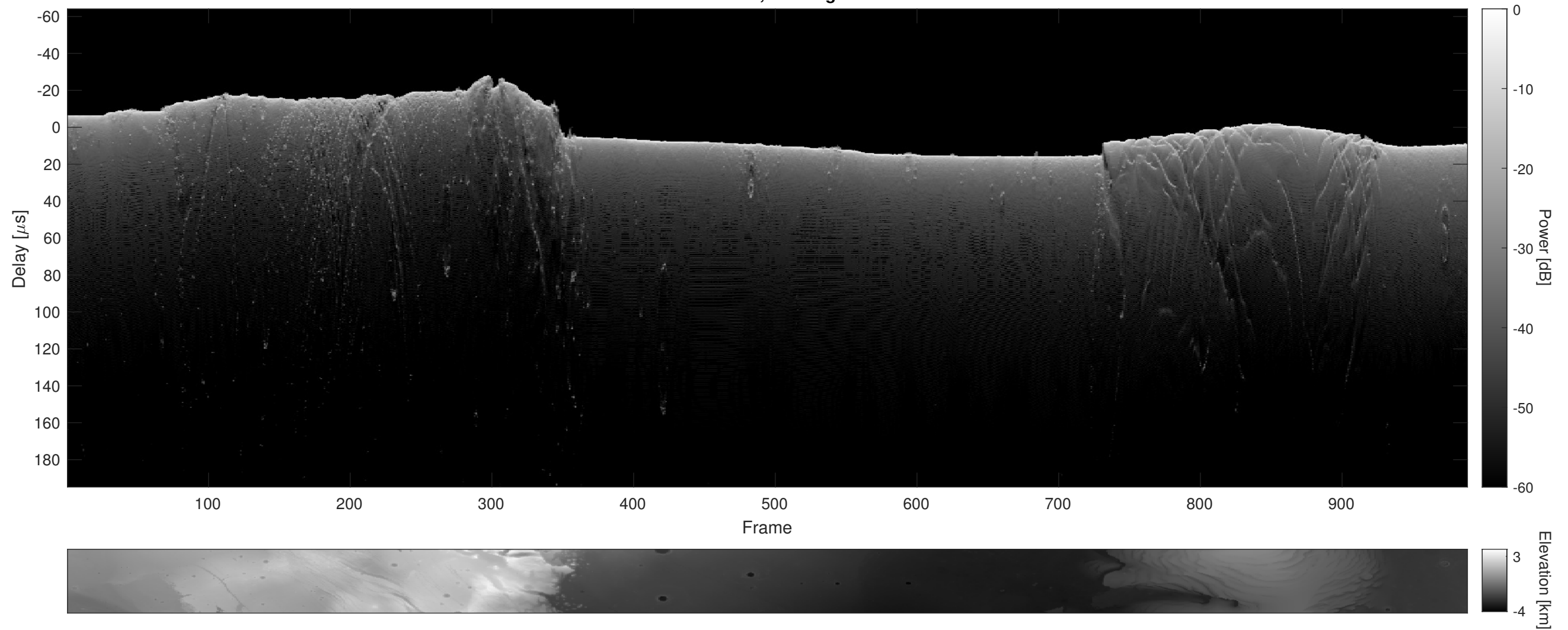
Orbit 22573, Cluttergram
