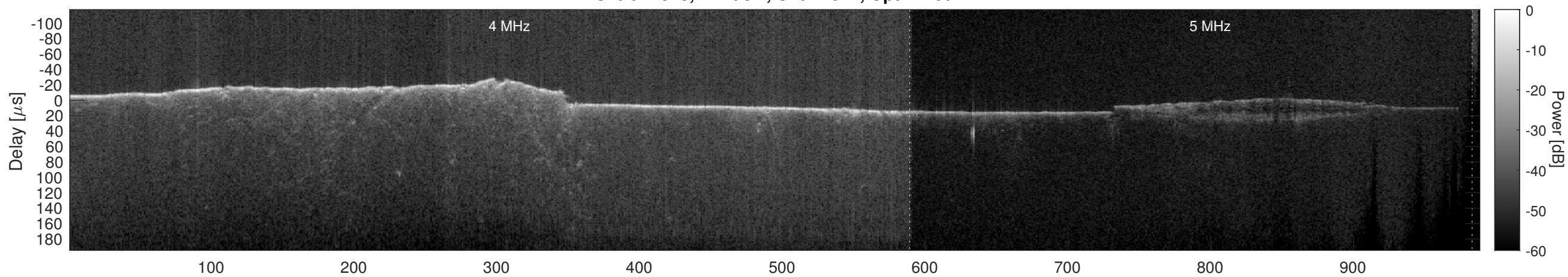
Orbit 22573, Cluttergram
