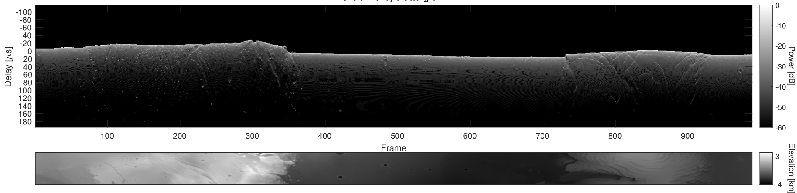
Orbit 22573, Cluttergram
