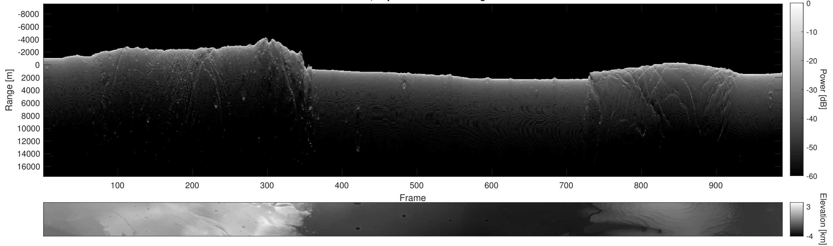
Orbit 22573, Depth-Corrected Cluttergram
