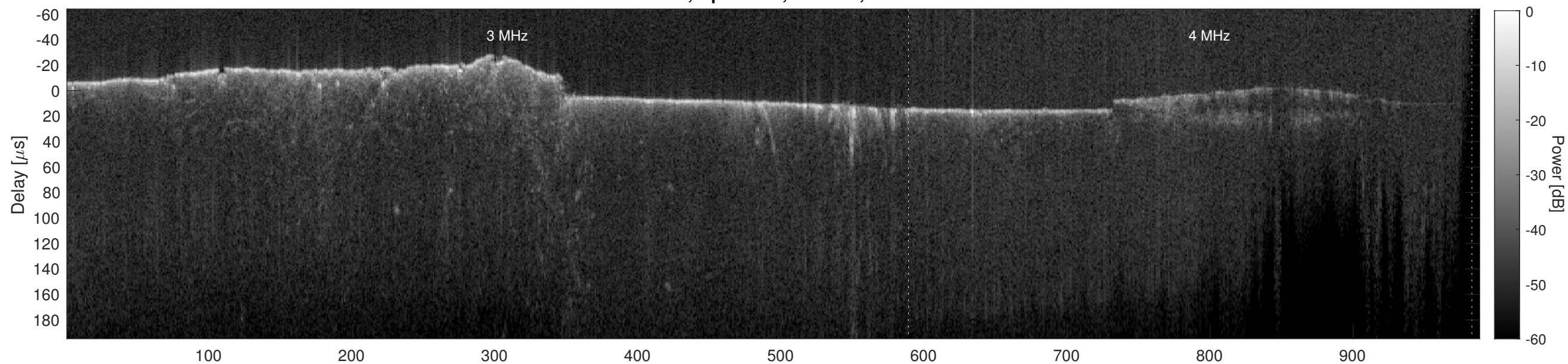
Orbit 22573, Cluttergram
