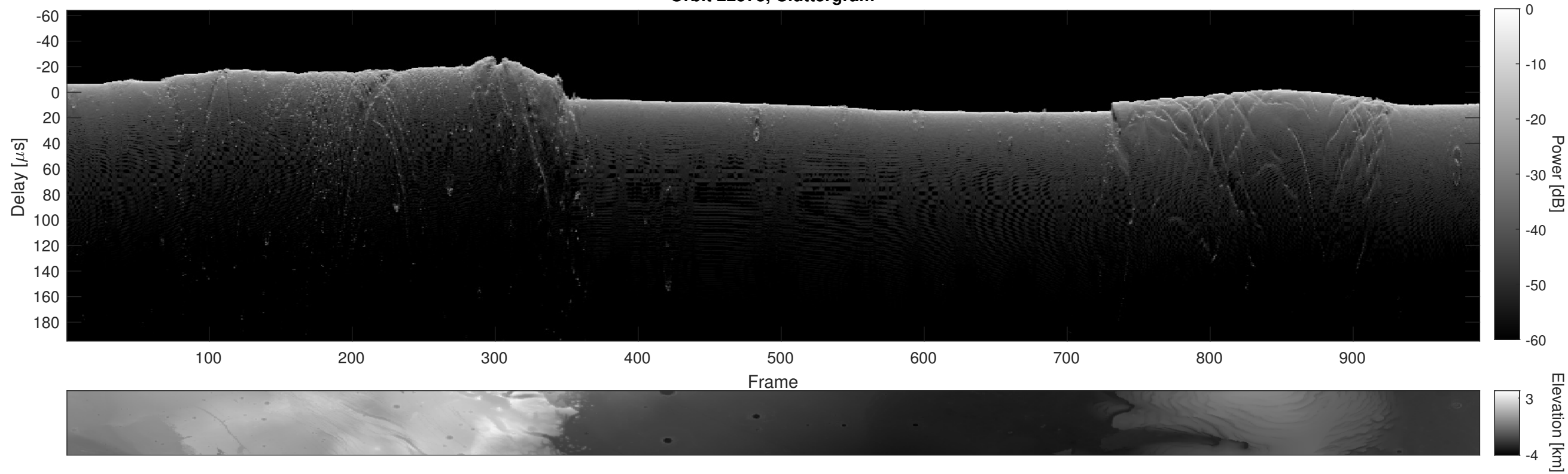
Orbit 22573, Cluttergram
