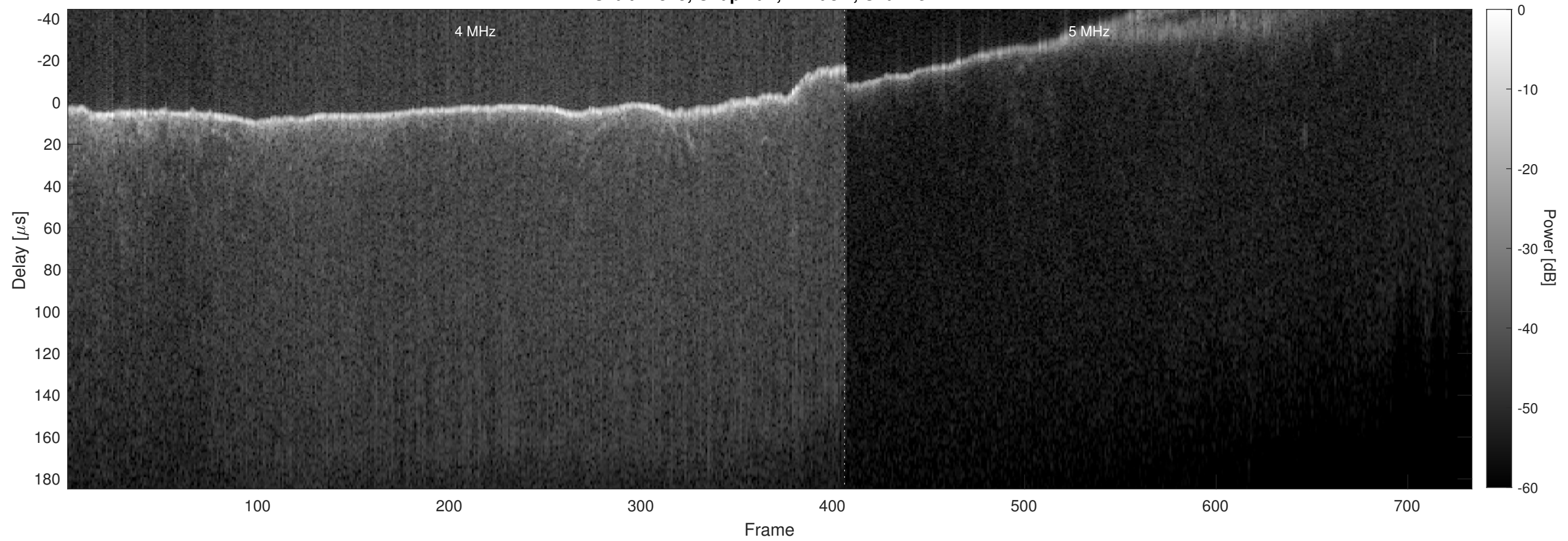
Orbit 22575, Chapman, Window, Channel 2
