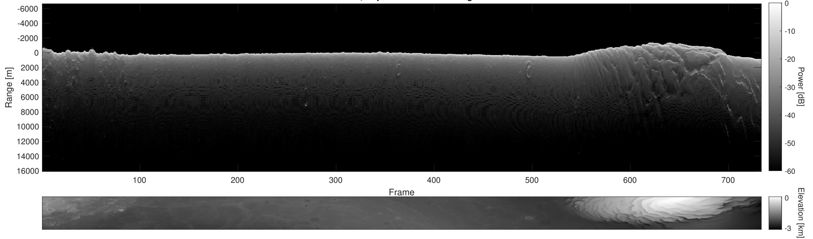
Orbit 22575, Depth-Corrected Cluttergram
