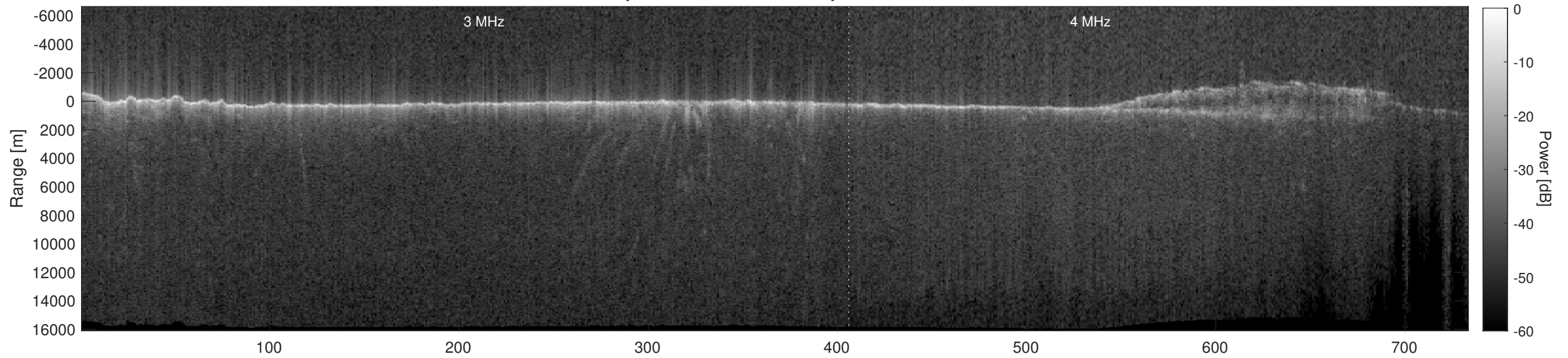
Orbit 22575, Depth-Corrected Cluttergram
