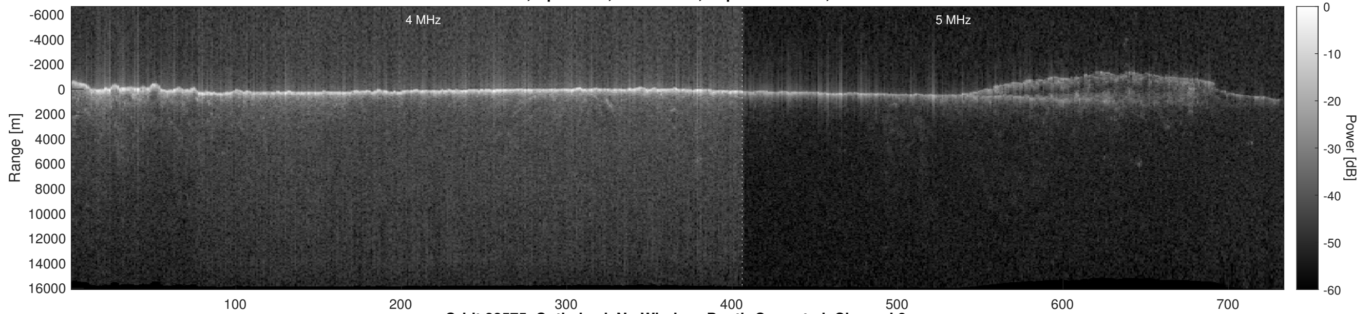
Orbit 22575, Optimized, No Window, Depth-Corrected, Channel 2
