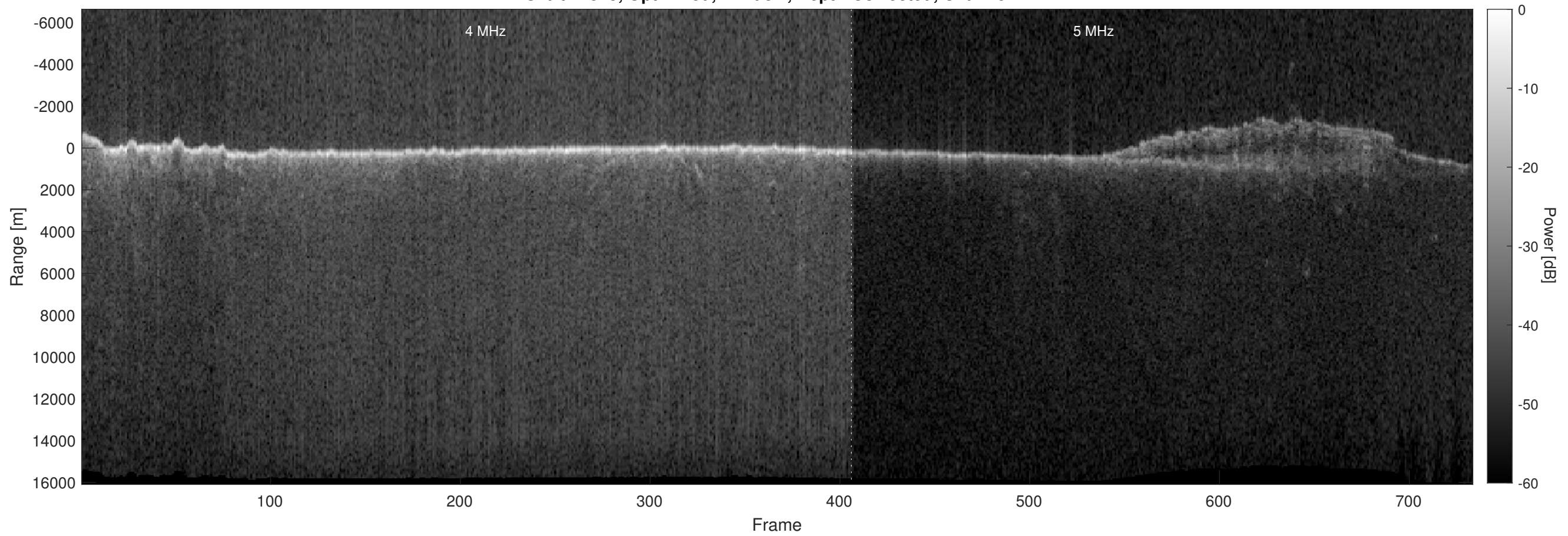
Orbit 22575, Optimized, Window, Depth-Corrected, Channel 2
