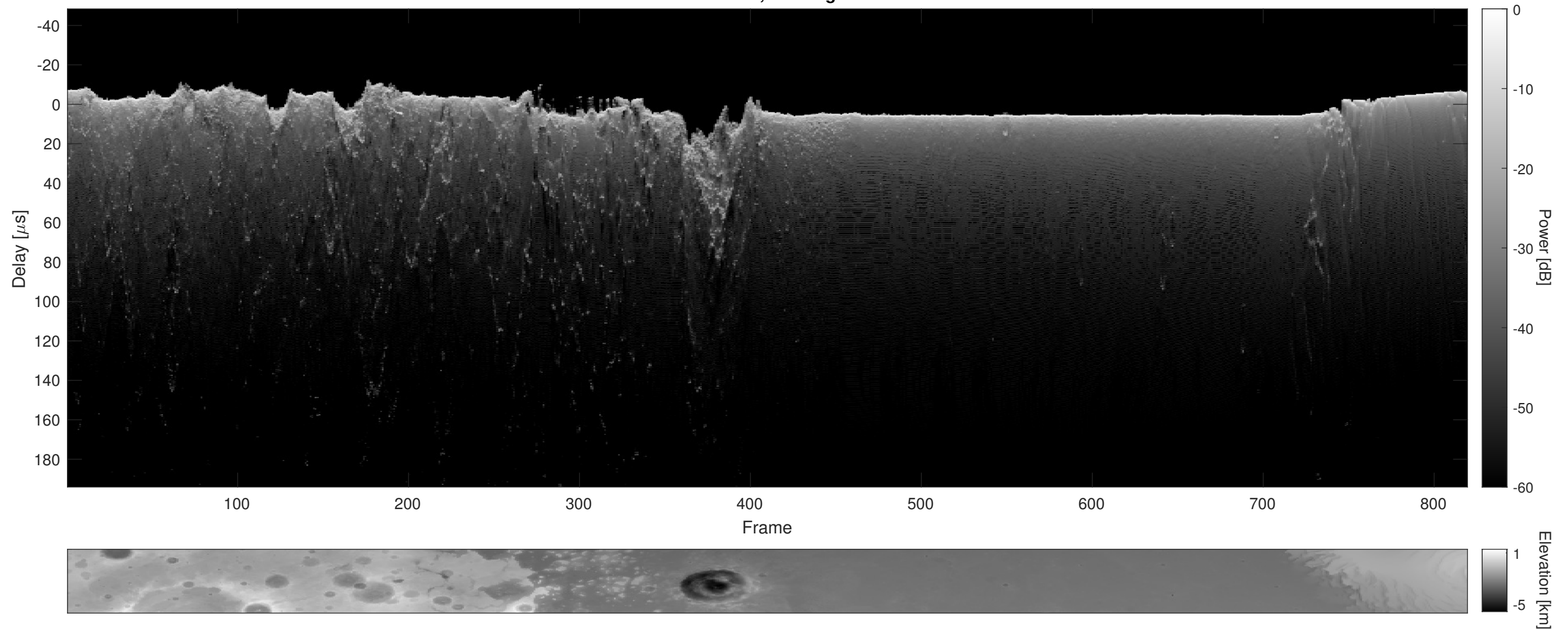
Orbit 22579, Cluttergram
