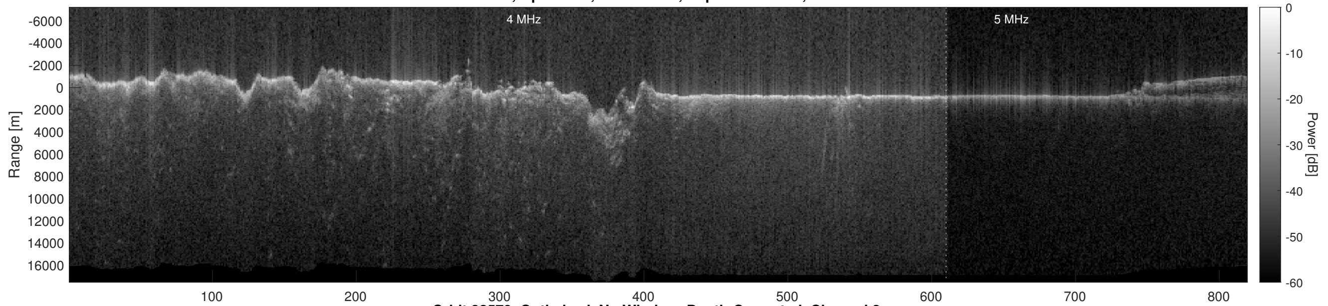
Orbit 22579, Optimized, No Window, Depth-Corrected, Channel 2
