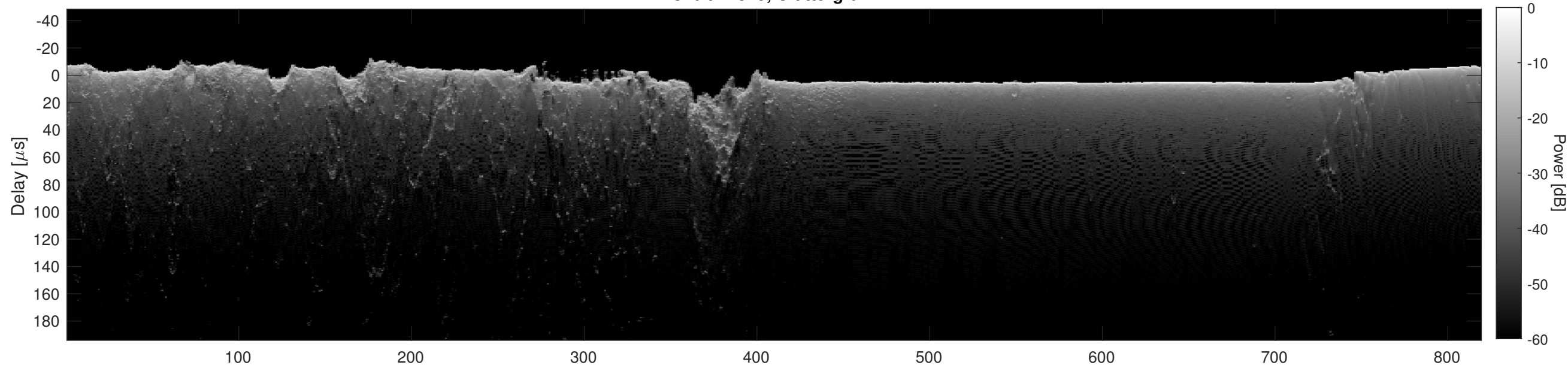
Orbit 22579, Cluttergram
