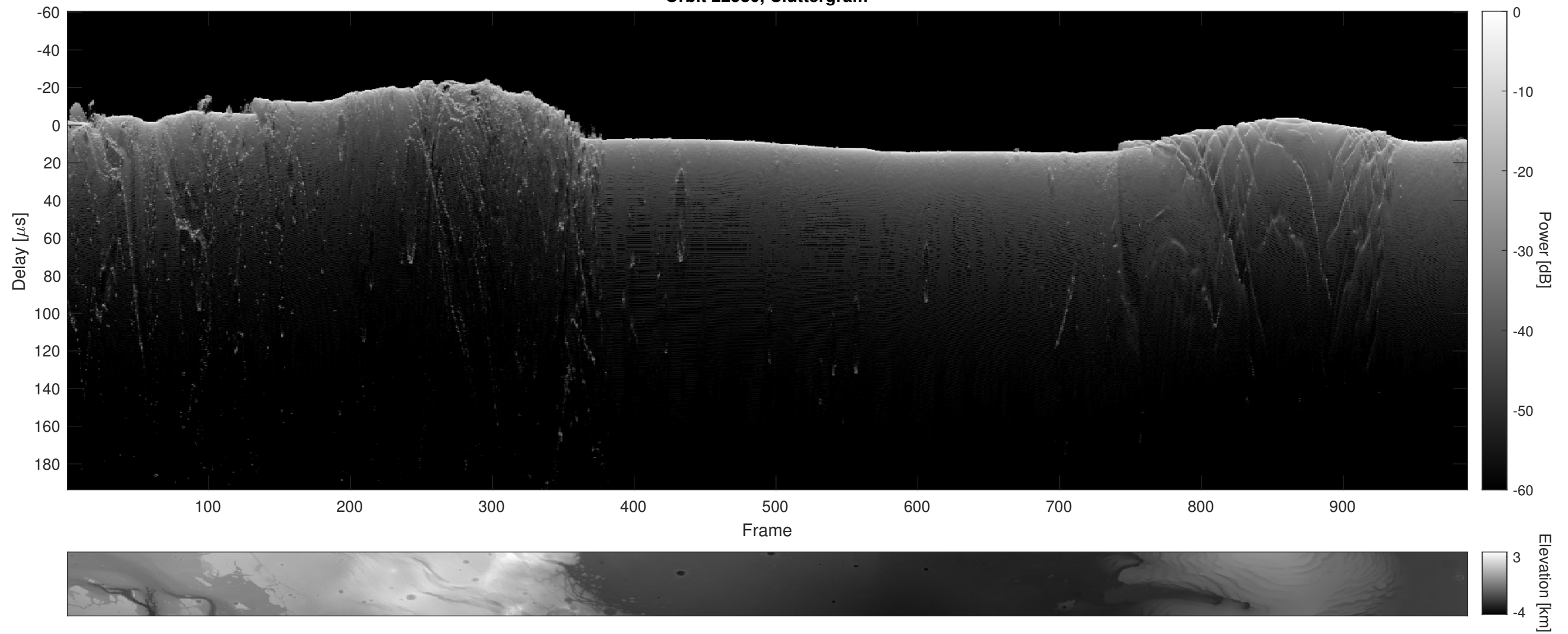
Orbit 22580, Cluttergram
