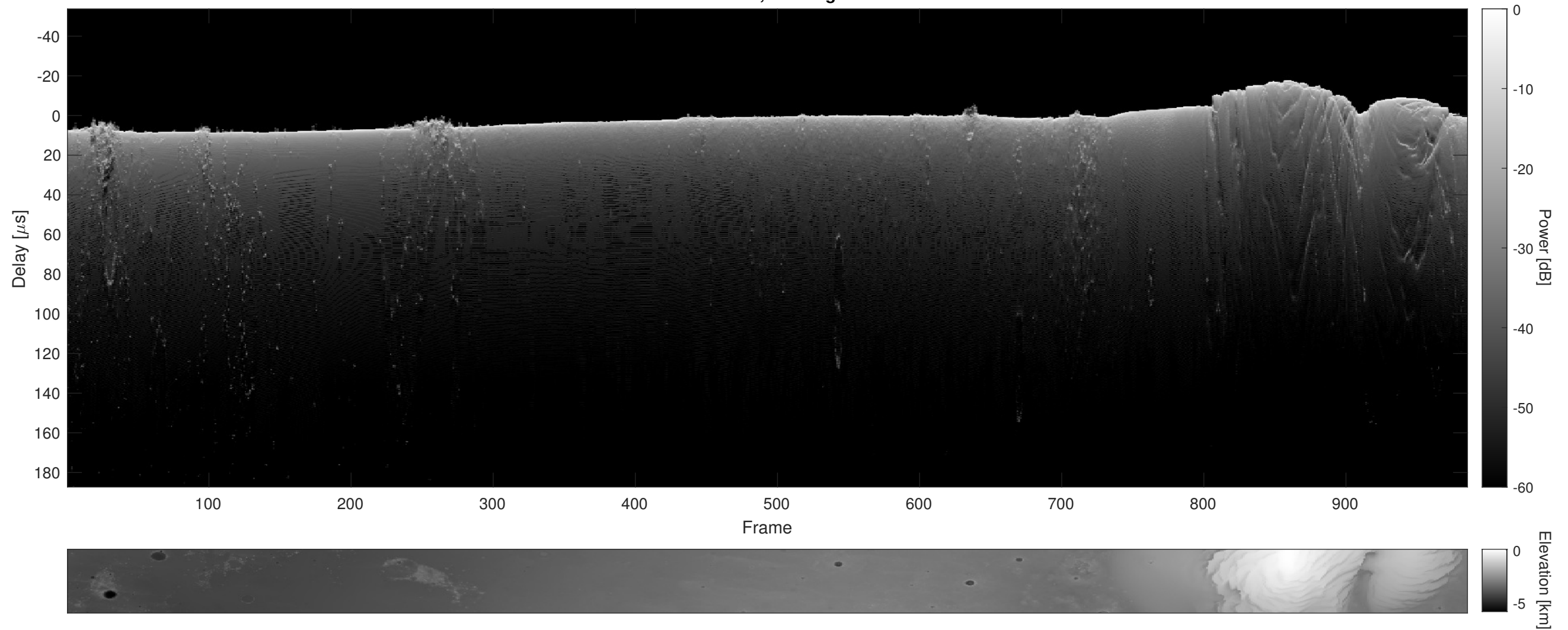
Orbit 22588, Cluttergram
