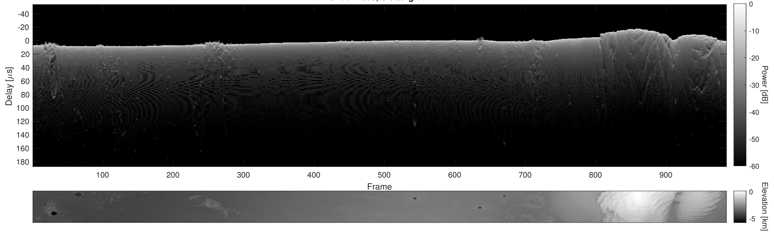
Orbit 22588, Cluttergram
