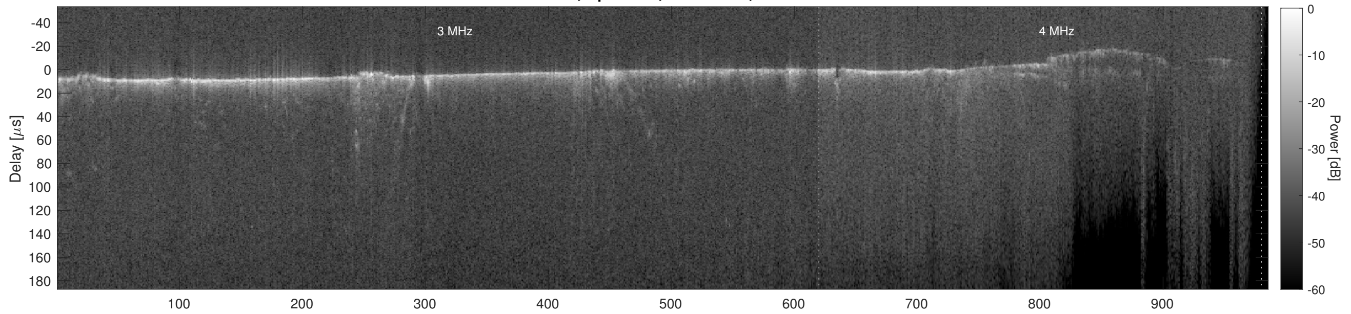
Orbit 22588, Cluttergram
