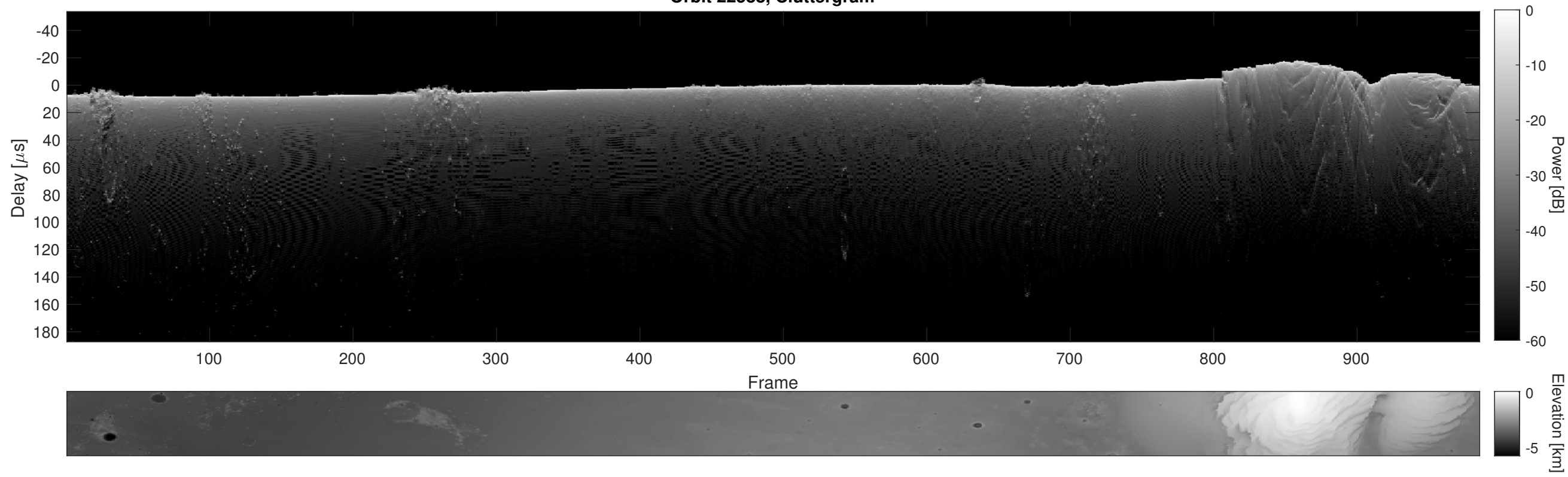
Orbit 22588, Cluttergram
