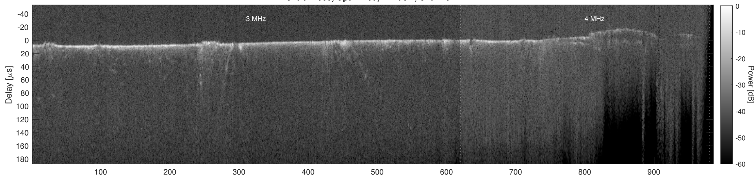
Orbit 22588, Cluttergram
