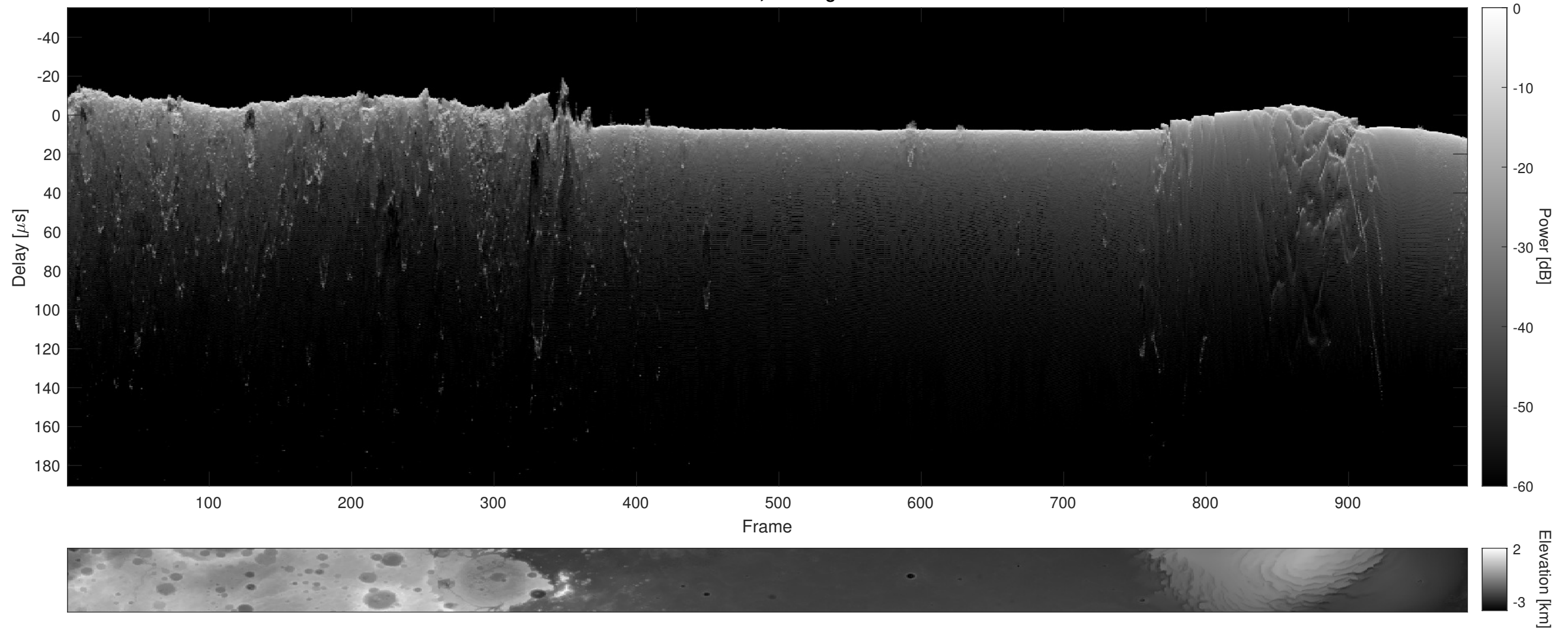
Orbit 22593, Cluttergram
