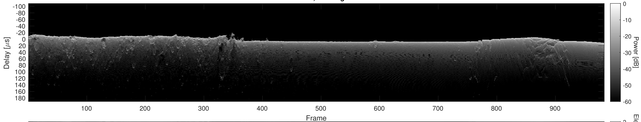
Orbit 22593, Cluttergram
