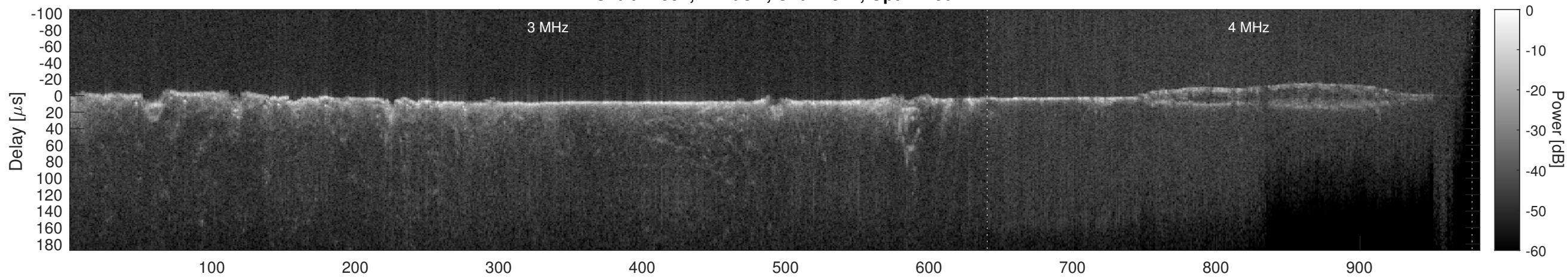
Orbit 22597, Cluttergram
